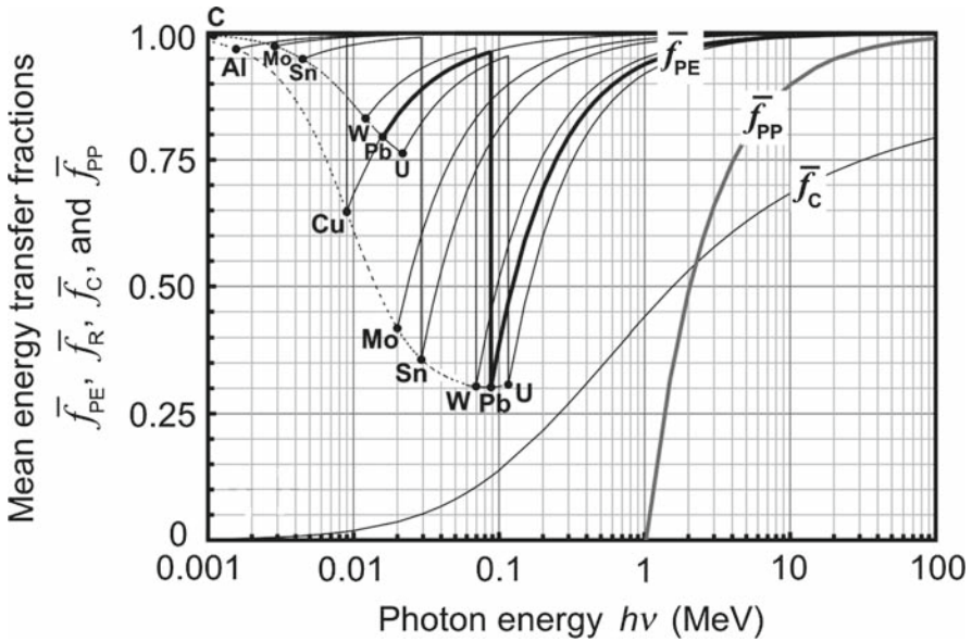
Fig. 8.2. Mean energy transfer fractions \bar{f}_i plotted against photon energy h\nu for the four main photon interactions with absorber atoms: \bar{f}_{\text{PE}} for photoelectric effect, \bar{f}_{\text{R}} for Rayleigh scattering, \bar{f}_{\text{C}} for Compton effect, and \bar{f}_{\text{PP}} for pair production. The photoelectric energy transfer fraction \bar{f}_{\text{PE}} depends on photon energy h\nu and on absorber atomic number Z , and is plotted for eight selected absorber atoms ranging from carbon to uranium. The energy transfer fractions for the other three effects: \bar{f}_{\text{R}} , \bar{f}_{\text{C}} , and \bar{f}_{\text{PP}} do not depend on absorber atomic number Z , therefore one curve for each effect covers all absorber atomic numbers. The dashed curves connect \bar{f}_{\text{PE}} points for which h\nu = E_{\text{B}}(\text{K}) and h\nu = E_{\text{B}}(\text{L}_1) . Note that \bar{f}_{\text{R}} = 0 for all photon energies h\nu and all absorber atomic numbers Z .
