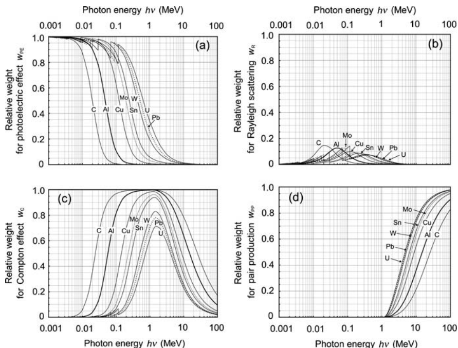
Fig. 8.4. Relative weights w_i for the four main photon interactions with atoms of absorber against photon energy h\nu for eight selected absorber atoms from carbon to uranium. (a) Relative weight of photoelectric effect w_{PE} ; (b) relative weight of Rayleigh scattering w_R ; (c) relative weight of Compton effect w_C ; and (d) relative weight of pair production w_{PP} . Data were calculated using the NIST XCOM database
