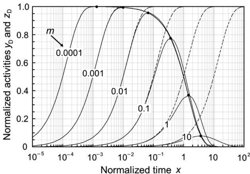
Fig. 12.3. Normalized daughter activities z_D of (12.35) for the saturation model (dashed curves) and y_D of (12.33) for the depletion model (solid curves) against the variable x for various activation factors m in the range from m = 10^{-4} to m = 10 . The heavy dots represent (y_D)_{\max} , the maxima of y_D for given m and follow the normalized parent activity y_P of (12.27). Variables x and y_P are given by (12.26) and (12.27), respectively. Variables z_D for the saturation model and y_D for the depletion model ( m \neq 1 ) are given by (12.35) and (12.33), respectively. Variable y_D for the depletion model with m = 1 is given by (12.34). The activation factor m is defined in (12.25)
