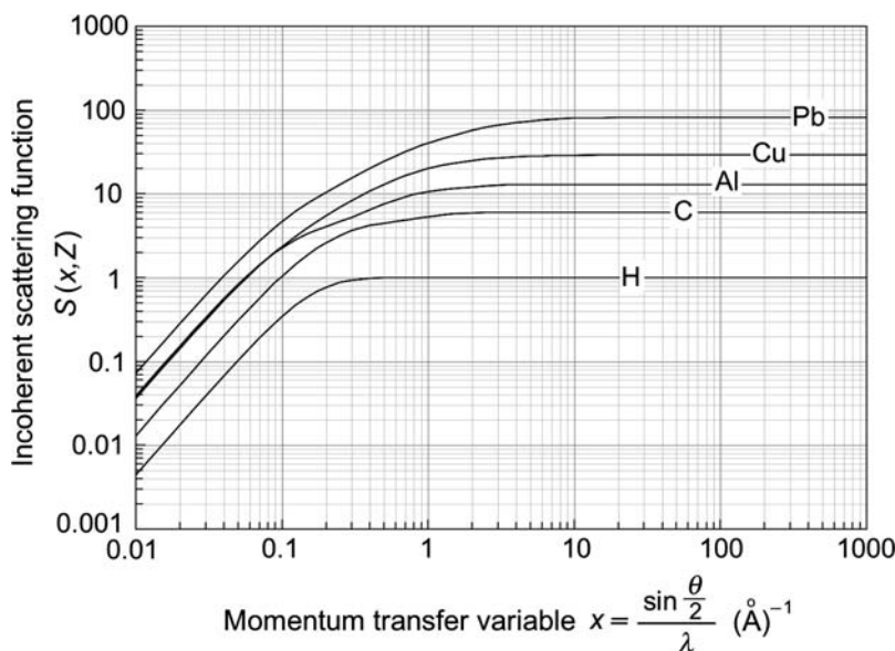
Fig. 7.20. Incoherent scattering function S(x, Z) plotted against the momentum transfer variable x where x = \sin(\theta/2)/\lambda for various absorbers in the range from hydrogen to lead. For large values of x the incoherent scattering function S(x, Z) saturates at Z , the atomic number of the absorber. The saturation values thus are: 1 for hydrogen; 6 for carbon; 29 for copper, and 82 for lead
