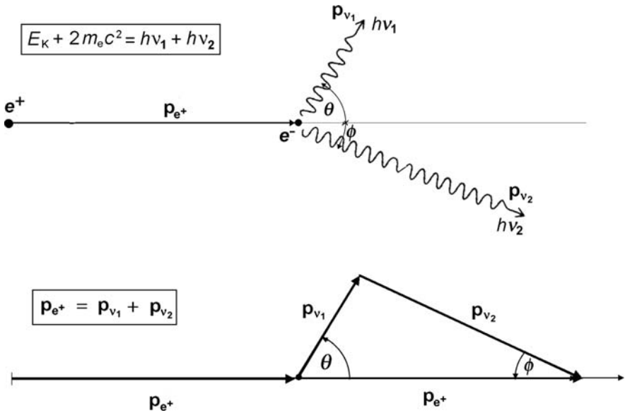
Fig. 7.39. Two-photon in-flight positron annihilation. The kinetic energy of the incident positron is E_K^{e^+} , its momentum is p_e = \sqrt{E_K^{e^+}(E_K^{e^+} + 2m_e c^2)} . Photon 1 is emitted with energy h\nu_1 and momentum \mathbf{p}_{\nu_1} ; photon 2 is emitted with energy h\nu_2 and momentum \mathbf{p}_{\nu_2} . The photon emission angles are \theta and \phi measured with respect to the direction of the incoming positron. The x components of \mathbf{p}_{\nu_1} and \mathbf{p}_{\nu_2} are h\nu_1 c^{-1} \cos \theta and h\nu_2 c^{-1} \cos \phi , respectively. The y components of \mathbf{p}_{\nu_1} and \mathbf{p}_{\nu_2} are h\nu_1 c^{-1} \sin \theta and h\nu_2 c^{-1} \sin \theta , respectively
