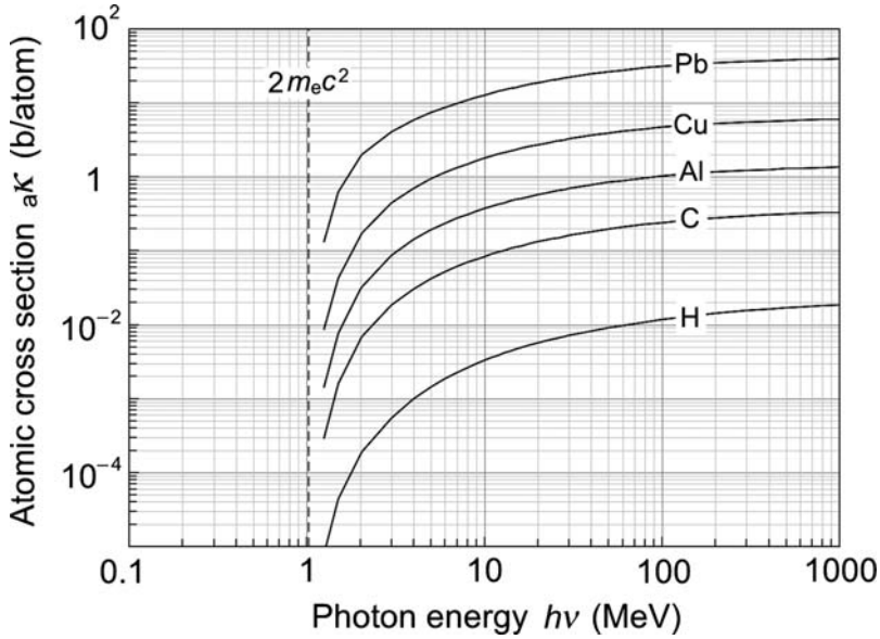
Fig. 7.36. Atomic cross section for general pair production (including nuclear pair production and triplet production) a\kappa against incident photon energy h\nu for various absorbers in the range from hydrogen to lead. Data are from the NIST
