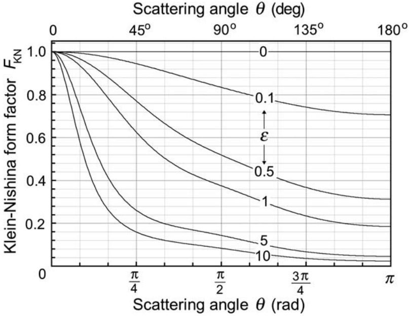
Fig. 7.12. Klein–Nishina atomic form factor for Compton effect F_{\text{KN}} against scattering angle \theta
