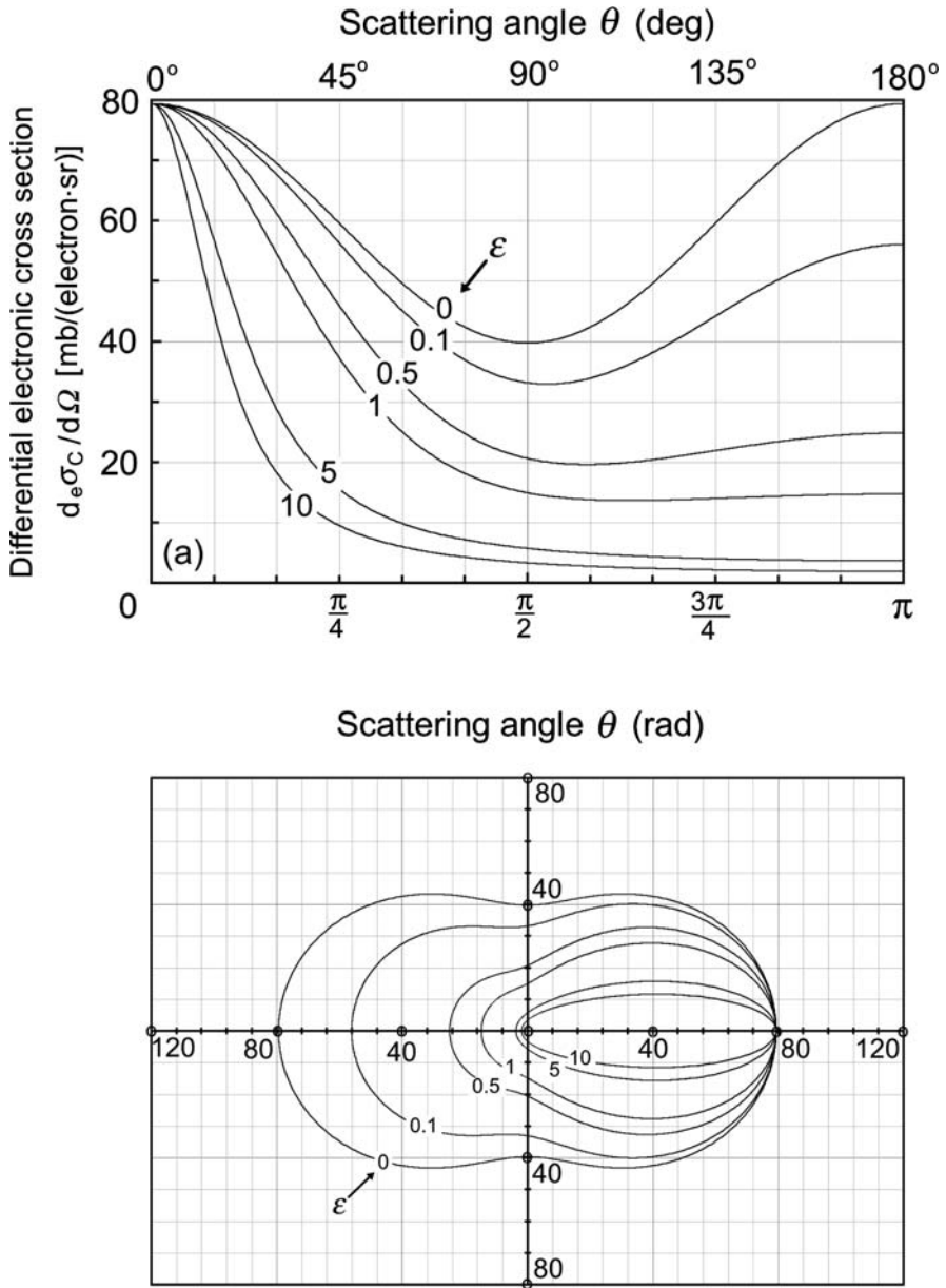
Fig. 7.13. Differential electronic cross section for Compton effect d_e \sigma_C^{\text{KN}} / d\Omega against scattering angle \theta for various values of \epsilon = h\nu / (m_e c^2) , as given by (7.89). The differential electronic cross section for Compton effect d_e \sigma_C^{\text{KN}} / d\Omega for \epsilon = 0 is equal to the differential electronic cross section for Thomson scattering d_e \sigma_{\text{Th}} / d\Omega (see Fig. 7.5). (a) Displays the data in Cartesian coordinate system; (b) in polar coordinate system
