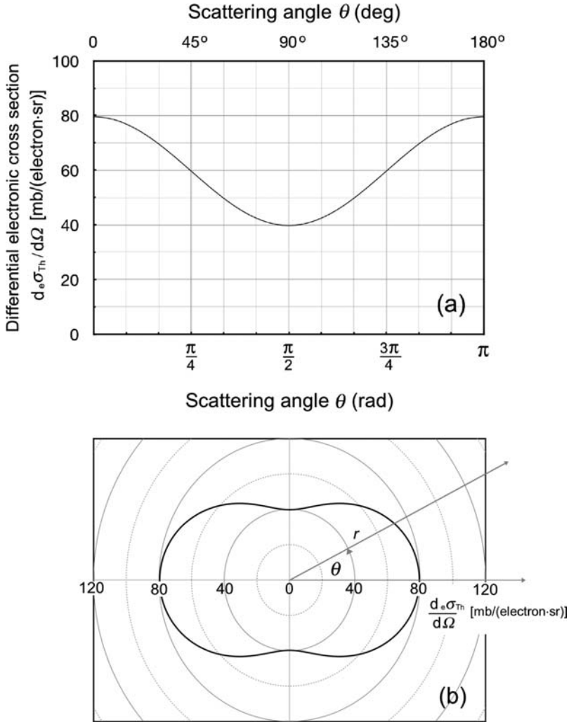
Fig. 7.5. Differential electronic cross section d_e \sigma_{Th}/d\Omega per unit solid angle against the scattering angle \theta for Thomson scattering, as given by (7.39). (a) Plotted in Cartesian coordinate system and (b) in polar coordinate system. The units shown are \text{mb}/(\text{electron} \cdot \text{steradian})
