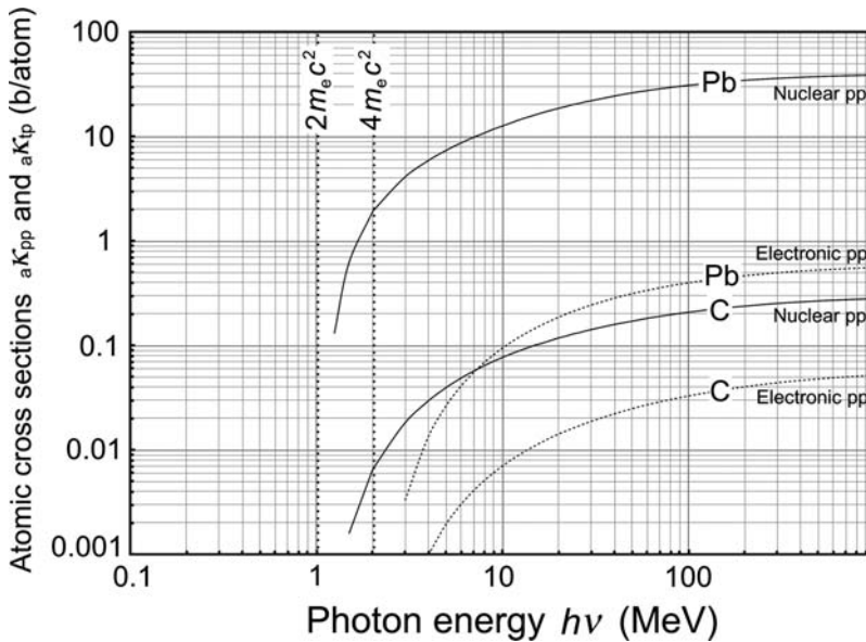
Fig. 7.35. Atomic cross sections for nuclear pair production {}_a\kappa_{\text{NPP}} (solid curves) and for triplet production (electronic pair production) {}_a\kappa_{\text{TP}} (dotted curves) against incident photon energy h\nu for carbon and lead. Data are from the NIST
