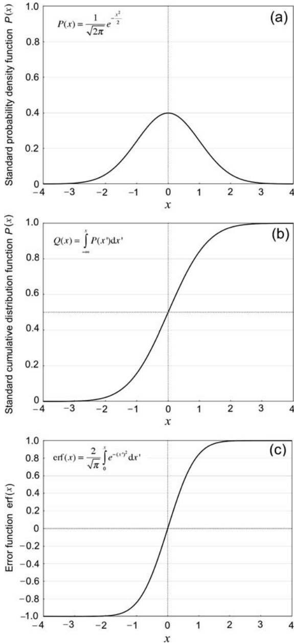
Fig. 1.12. Part a : Standard probability density function P(x) of (1.142) for the mean or expectation value \bar{x} = 0 ; standard deviation \sigma = 1 , and variance v = 1 . Part b : Standard cumulative distribution function Q(x) of (1.158) for the mean or expectation value \bar{x} = 0 ; standard deviation \sigma = 1 , and variance v = 1 . Part c : Error function \text{erf}(x) of (1.159).
