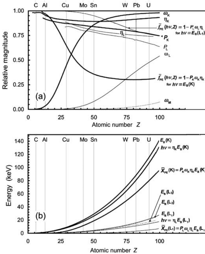
Fig. 7.29. Various atomic parameters relevant to photoelectric effect plotted against atomic number Z of the absorber: (a) fluorescence yields \omega_K , \omega_L , and \omega_M ; photoelectric probabilities P_K and P_L ; fluorescence efficiencies \eta_K and \eta_L , and photoelectric mean energy transfer fractions \bar{f}_{PE} for photon energies h\nu = E_B(K) and h\nu = E_B(L_1) . (b) K-shell and L_1 , L_2 , L_3 -subshell binding energies; mean fluorescence photon energies h\nu_K and h\nu_L ; and mean fluorescence emission energies \bar{X}_{PE}(K) and \bar{X}_{PE}(L_1)
