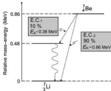
Fig. 11.7. Decay scheme for electron capture decay of berillium-7 into lithium-7. The relative mass-energy levels for the ground states of the two nuclides are calculated from the respective atomic masses listed in Appendix A
