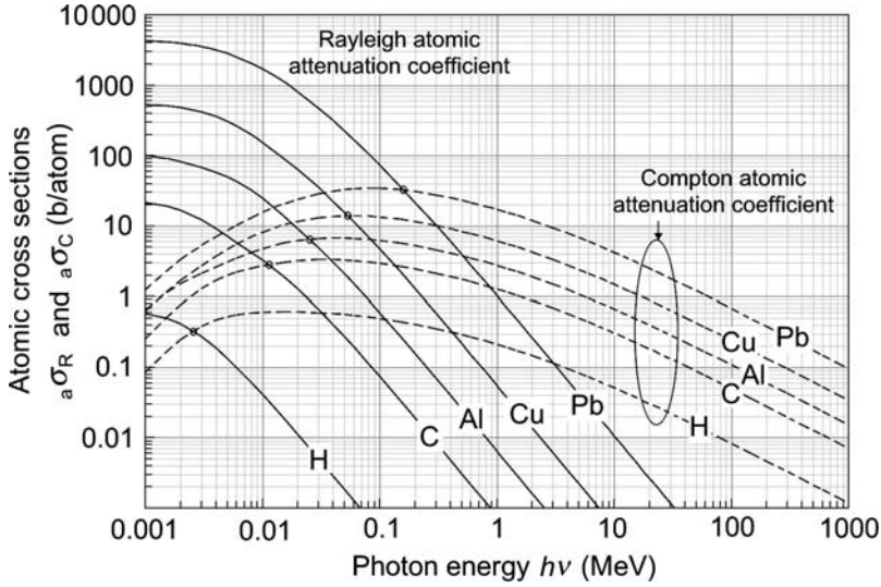
Fig. 7.25. Atomic cross sections for Rayleigh scattering \sigma_R shown with solid curves and atomic cross sections for Compton scattering \sigma_C shown with dashed curves against incident photon energy h\nu in the range from 1 keV to 1000 MeV for various absorbers ranging from hydrogen to lead. For very low photon energies \sigma_R curves exhibit a plateau with a value of \sigma_{Th}Z^2 where \sigma_{Th} is the energy independent Thomson cross section and Z is the atomic number of the absorber (note that F(x, Z) \rightarrow Z for low h\nu , i.e., large \lambda ). For a given absorber, the photon energy h\nu_{eq} at which \sigma_R = \sigma_C is indicated with o. Data are from the NIST
