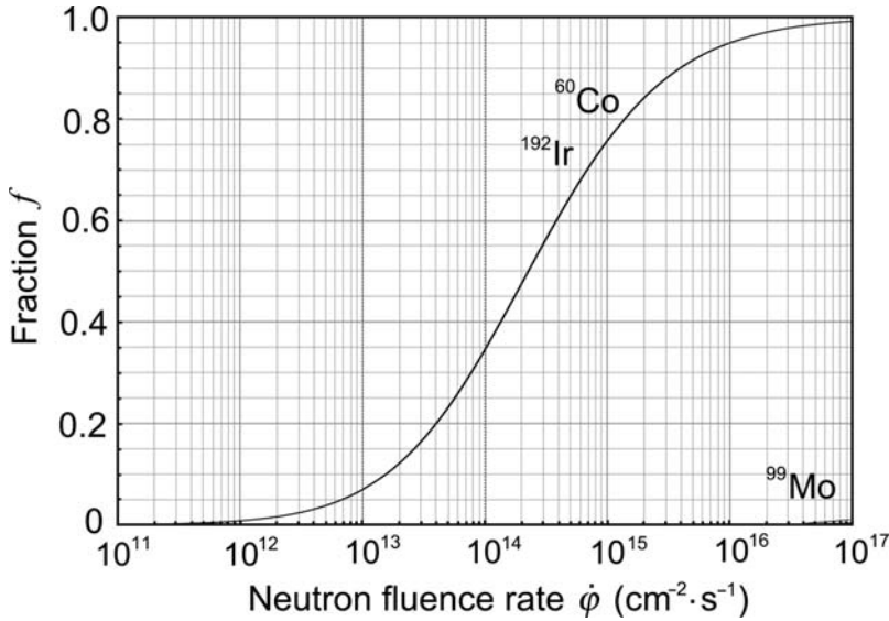
Fig. 12.7. Specific activity fraction f defined as (a_D)_{\max} / (a_D)_{\text{theor}} plotted against the neutron fluence rate \dot{\phi} for cobalt-60, iridium-192, and molybdenum-99. The data for molybdenum are visible only at very high fluence rates because the activation factor m at a given \dot{\phi} is several orders of magnitude smaller for molybdenum-99 in comparison with that of cobalt-60 and iridium-192
