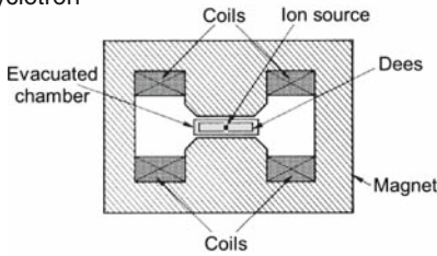
(b) Cyclotron
