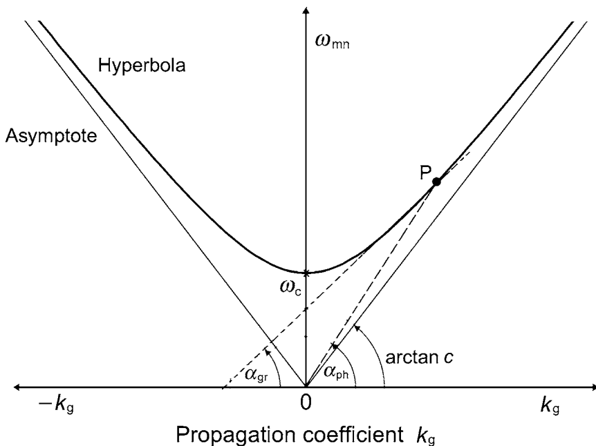
Fig. 13.3. Hyperbolic dispersion relationship ( \omega - k_g ) for a uniform waveguide. Point P is an arbitrary point on the dispersion \omega - k_g curve. Angles \alpha_{ph} and \alpha_{gr} are shown for point P. The asymptotes of the dispersion hyperbola form an angle \arctan c with the abscissa ( k_g ) axis
