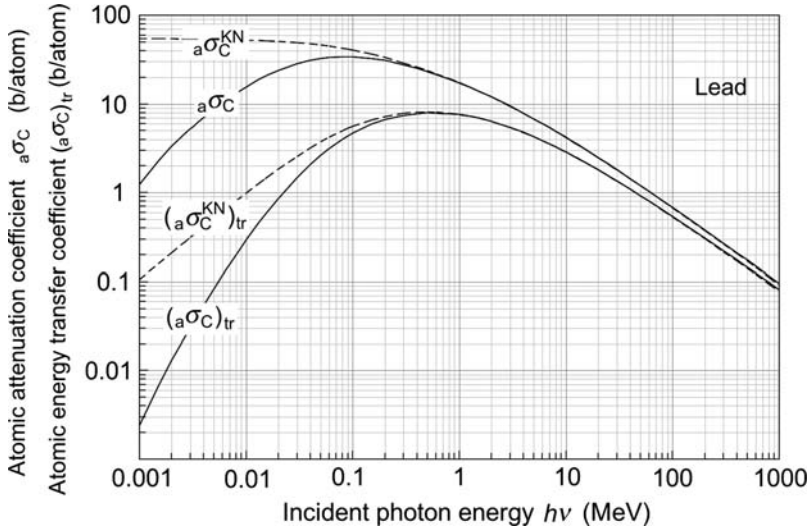
Fig. 7.22. The Compton atomic attenuation coefficient (cross section) for lead of Fig. 7.19 and the Compton atomic energy transfer coefficients for lead; dashed curves are Klein–Nishina data for free unbound electrons; solid curves are data incorporating electronic binding effects. Data are from the NIST
