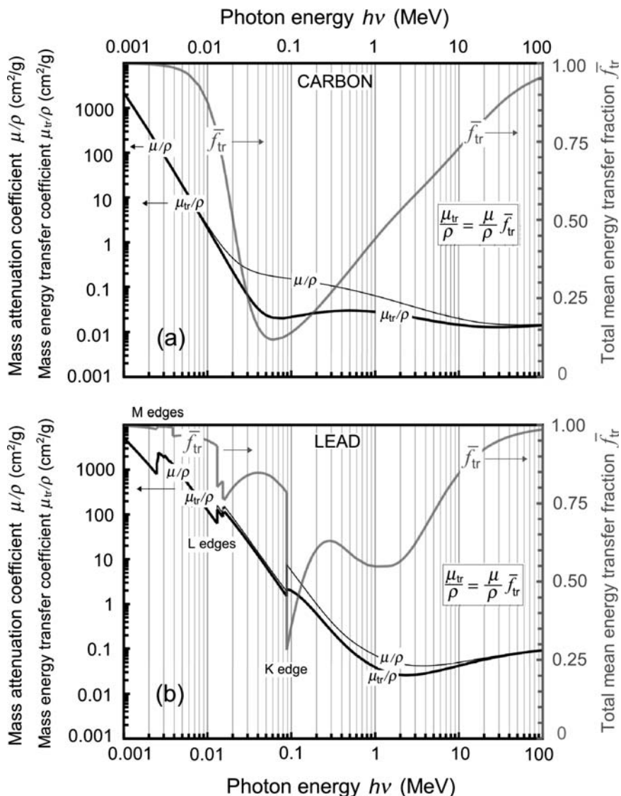
Fig. 8.9. Mass attenuation coefficient \mu/\rho from the NIST XCOM database and the calculated mass energy transfer coefficient \mu_{tr}/\rho against photon energy h\nu for carbon in (a) and lead in (b). Values of the two coefficients are given in \text{cm}^2/\text{g} in the left hand scale. The total mean energy transfer fraction \bar{f}_{tr} of (8.5) which links \mu_{tr}/\rho with \mu/\rho is shown in the background with values shown on the right hand scale. The attenuation coefficient \mu/\rho is plotted with the fine dark line, the energy transfer coefficient \mu_{tr}/\rho with the heavy dark line, and the total energy transfer fraction \bar{f}_{tr} with the light grey line
