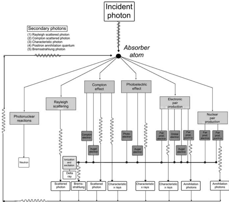
Fig. 8.18. Schematic diagram of the six modes available to incident photons for interaction with absorber atoms of importance to medical physics: photonuclear reactions, Rayleigh scattering, Compton effect, photoelectric effect, electronic pair production, and nuclear pair production (Note: the modes are not listed in any particular order of importance). Also shown are the particles produced or released in the absorber during a given photon interaction as well as the effects that follow a given photon interaction, such as emission of characteristic radiation, Auger electrons, annihilation quanta, and bremsstrahlung photons. Figure also indicates that the secondary photons (Rayleigh- and Compton-scattered photons, characteristic photons, annihilation quanta, and bremsstrahlung photons) can start their own photon interaction cycle in the absorber
