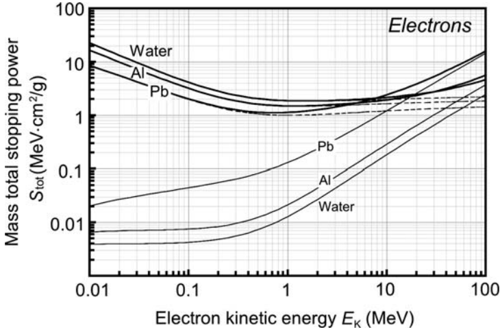
Fig. 6.11. Total mass stopping power S_{\text{tot}} for electrons in water, aluminum and lead against the electron kinetic energy shown with heavy solid curves. The mass collision stopping powers and mass radiation stopping powers are shown with dashed curves and light solid curves, respectively, for comparison. The total stopping power of a given material is the sum of the radiation and collision stopping powers. Data were obtained from the NIST. The critical energies (E_K)_{\text{crit}} are 100 MeV, 61 MeV, and 10 MeV for water, aluminum, and lead, respectively
