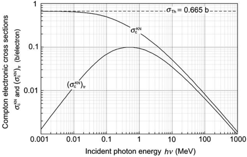
Fig. 7.17. Compton electronic cross section {}_e\sigma_C^{KN} and Compton electronic energy transfer cross section ({}_e\sigma_C^{KN})_{tr} for a free electron against incident photon energy h\nu in the energy range from 0.001 MeV to 1000 MeV, determined from Klein–Nishina equations given in (7.104) and (7.108), respectively. For very low photon energies, {}_e\sigma_C^{KN} \approx {}_e\sigma_{Th} = 0.665 \text{ b} . For very high photon energies ( h\nu \rightarrow \infty ), ({}_e\sigma_C^{KN})_{tr} \approx {}_e\sigma_C^{KN}
