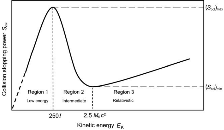
Fig. 6.7. Schematic representation of the shape of the collision stopping power S_{\text{col}} as a function of the charged particle kinetic energy E_K . Three regions are shown as the kinetic energy increases from zero: (1) low energy region; (2) intermediate energy region; and (3) relativistic energy region. In region (1), S_{\text{col}} rises almost linearly and reaches a maximum at about 250 I , where I is the mean ionization/excitation potential of the absorber. In region (2), S_{\text{col}} decreases as 1/v^2 or 1/E_K where v is the velocity of the charged particle to reach a broad minimum at \sim 2.5 M_0 c^2 where M_0 c^2 is the rest energy of the charged particle. In region (3), S_{\text{col}} rises slowly with increasing E_K because of relativistic effects
