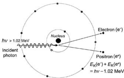
Fig. 8.17. Schematic diagrams of the six most important modes of photon interaction with atoms of absorber: a Photoelectric effect; b Rayleigh scattering; c Compton effect; d Electronic pair production (triplet production); e Nuclear pair production; f Photodisintegration. The first four modes represent photon interactions with a K-shell orbital electron; the last two modes ( e and f ) represent photon interactions with the nucleus of the absorber atom. The electronic and nuclear pair production modes are usually handled together under the header “pair production”, and photonuclear reactions are usually ignored, so that often in medical physics an assumption is made that there are only four important modes of photon interaction with absorber atoms: photoelectric effect, Rayleigh scattering, Compton effect, and pair production.
