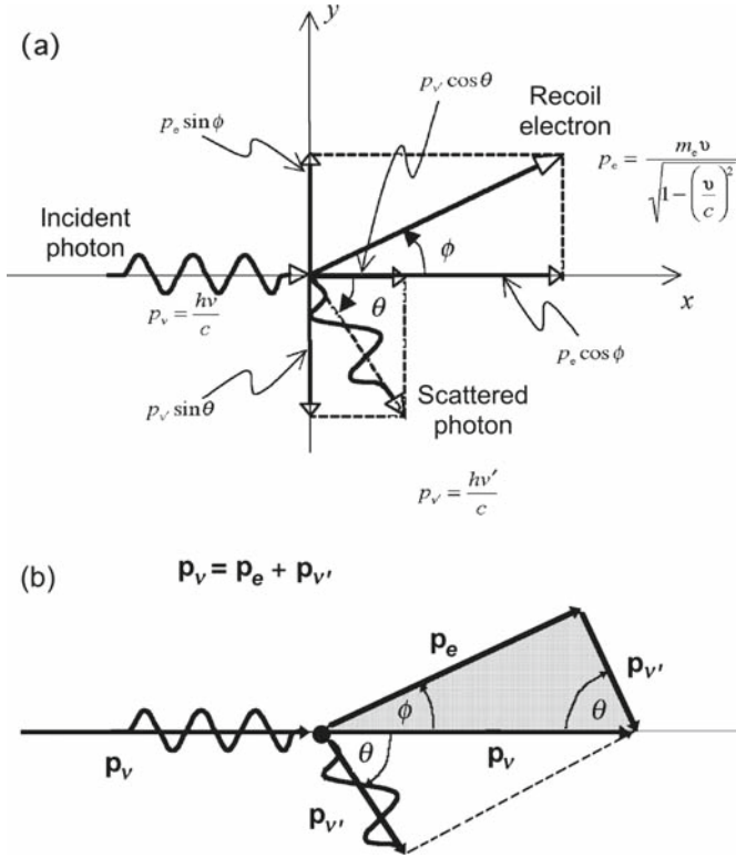
Fig. 7.7. Diagram of Compton effect. An incident photon with energy h\nu = 1 \text{ MeV} interacts with a stationary and free electron. A photon with energy h\nu' is produced and scattered with a scattering angle \theta = 60^\circ . The difference between the incident photon energy h\nu and the scattered photon energy h\nu' is given as kinetic energy to the recoil electron. (a) Schematic diagram; (b) vector representation of the effect
