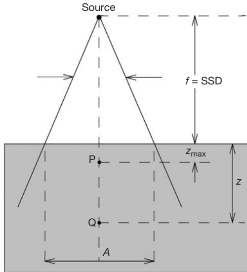
FIG. 6.9. Geometry for PDD measurement and definition. Point Q is an arbitrary point on the beam central axis at depth z , point P is the point at z_{\max} on the beam central axis. The field size A is defined on the surface of the phantom.
