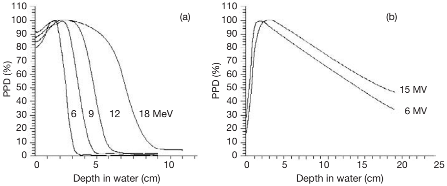
FIG. 8.1. Typical central axis PDD curves in water for a 10 \times 10 \text{ cm}^2 field size and an SSD of 100 cm for (a) electron beams with energies of 6, 9, 12 and 18 MeV and (b) photon beams with energies of 6 and 15 MV.
