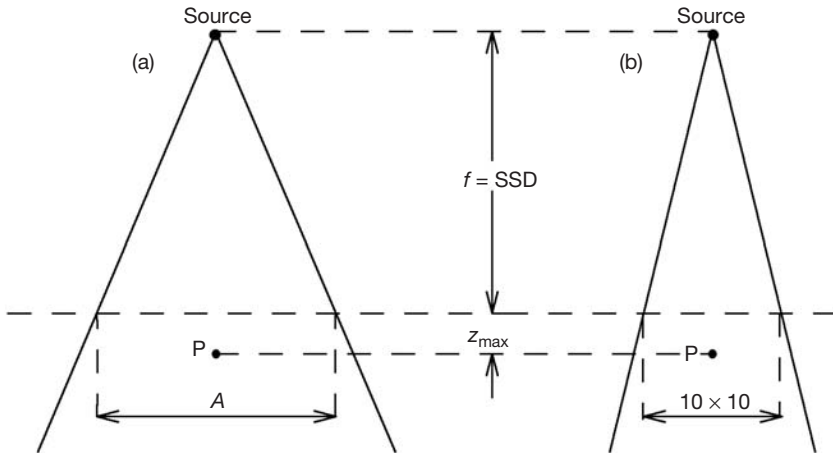
FIG. 6.4. Geometry for measurement of CF(A, hv) . The ‘dose to small mass of water’ is measured at point P in air: in part (a) with field size A , in part (b) with field size 10 \times 10 \text{ cm}^2 . Parameter f stands for the SSD.
