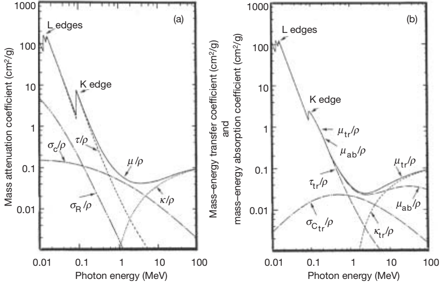
FIG. 1.7. Mass attenuation coefficient \mu/p (a); mass–energy transfer coefficient \mu_{tr}/p and mass–energy absorption coefficient \mu_{ab}/p (b) for lead in the photon energy range between 10 keV and 100 MeV. The dotted–dashed curves represent contributions of individual effects, while the solid curves represent the sum of the contributions of the individual effects as given by Eq. (1.88) for \mu/p , Eq. (1.89) for \mu_{tr}/p and Eq. (1.90) for \mu_{ab}/p . For photon energies below 2 MeV, \mu_{tr}/p \approx \mu_{ab}/p , because the radiative fraction g in this energy region is negligible. Above 2 MeV, g increases with photon energy, causing the divergence between the mass–energy transfer and mass–energy absorption coefficients.
