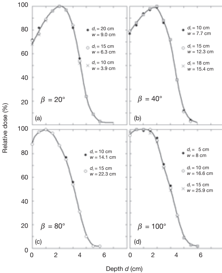
FIG. 8.11. Radial PDDs in electron arc therapy measured in a phantom for various combinations of w and d_p , giving characteristic angles \beta of (a) 20^\circ , (b) 40^\circ , (c) 80^\circ and (d) 100^\circ . The electron beam energy is 9 MeV.
