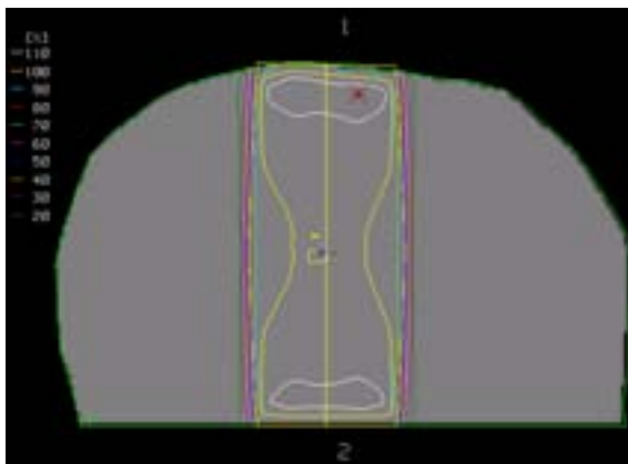
FIG. 7.21. A parallel opposed beam pair is incident on a patient. Note the large rectangular area of relatively uniform dose ( <15\% variation). The isodoses have been normalized to 100% at the isocentre. This beam combination is well suited to a large variety of treatment sites (e.g. lung, brain, head and neck).
