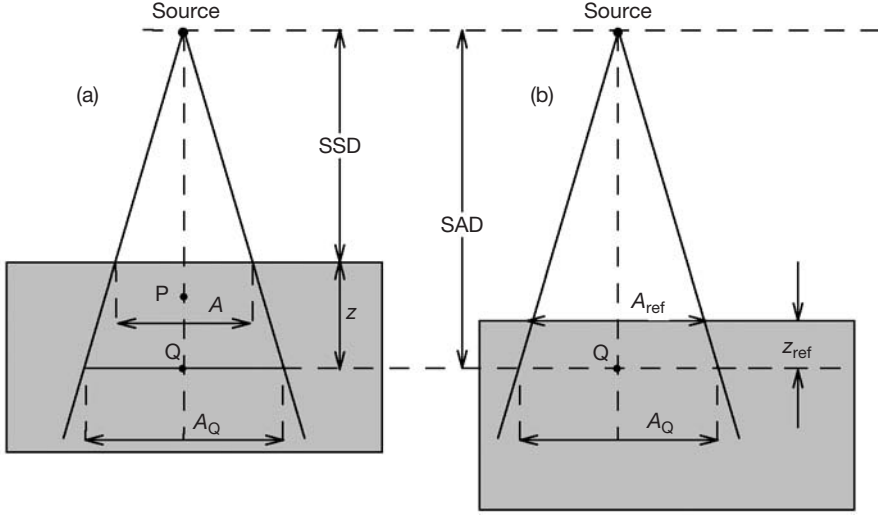
FIG. 6.15. Geometry for measurement of TPR(d, A_Q, hv) . (a) The geometry for the measurement of D_Q at depth z in a phantom; (b) the geometry for the measurement of D_{Qref} at depth z_{ref} in a phantom. The distance between the source and the point of measurement, as well as the field size at the point of measurement, is the same for (a) and (b).
