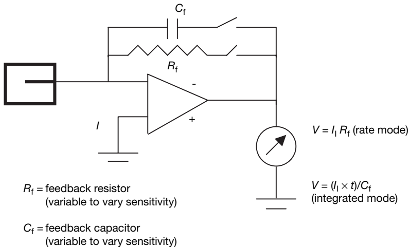
FIG. 3.3. Electrometer in feedback mode of operation.
