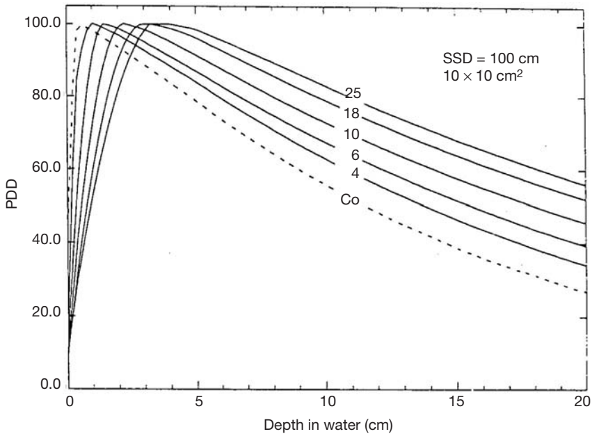
FIG. 6.10. PDD curves in water for a 10 \times 10 \text{ cm}^2 field at an SSD of 100 cm for various megavoltage photon beams ranging from ^{60}\text{Co} \gamma rays to 25 MV X rays.
