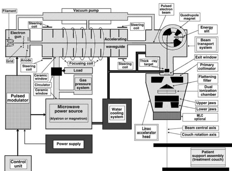
FIG. 5.4. Medical linac.
