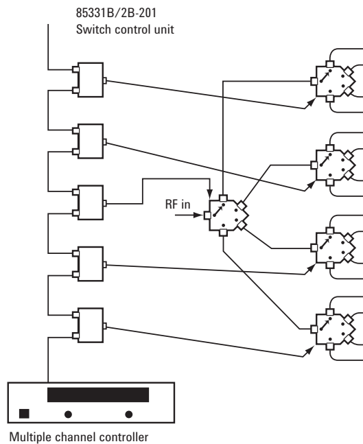
Figure 54. Example 1P16T switch configuration constructed from modular components.
