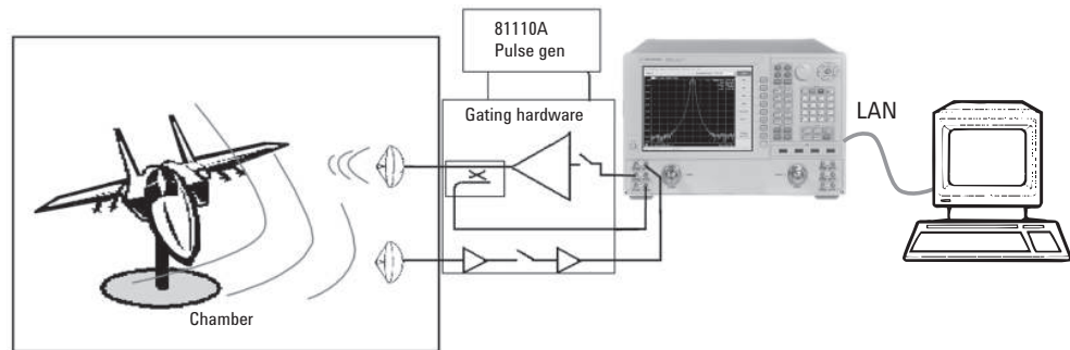
Figure 8. Typical RCS measurement configuration using a PNA Option 201, PNA-X network analyzer.
