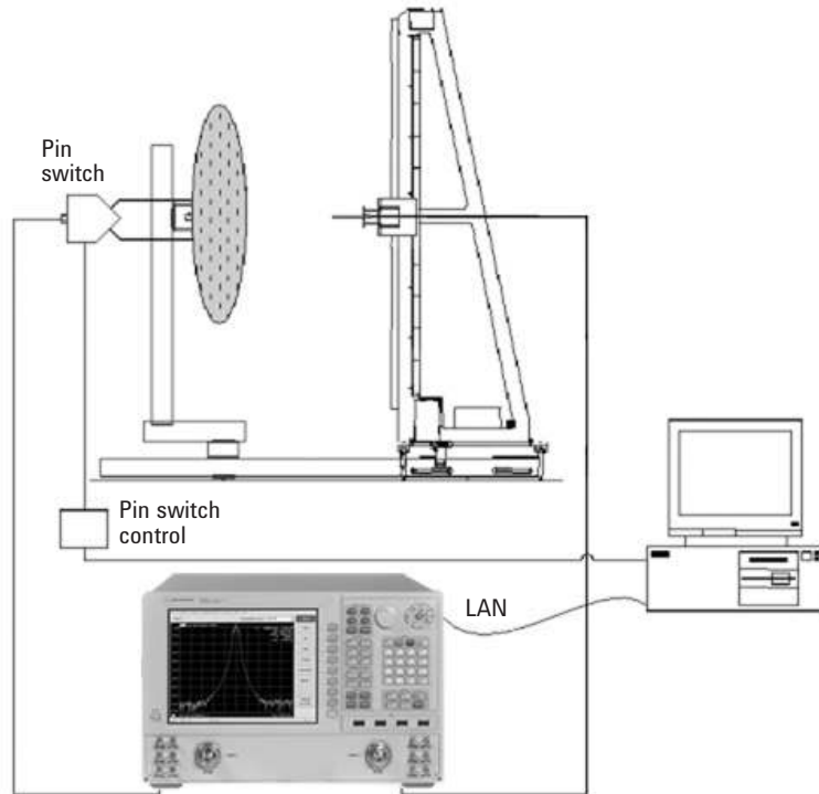
Figure 2. Typical near-field antenna measurement configuration using a PNA/PNA-X. In addition, PNA-L with direct receiver access can be used.
