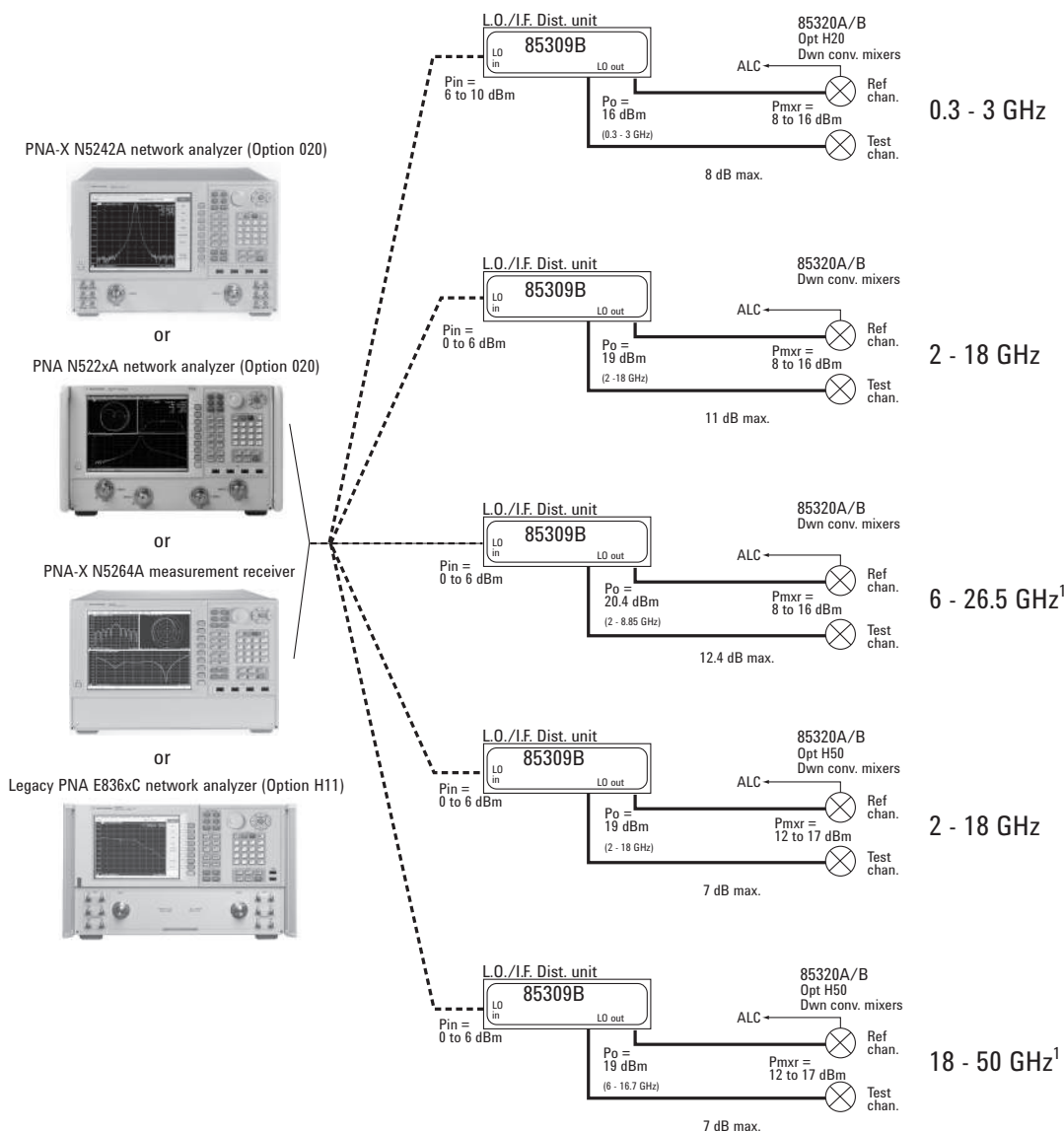
Figure 39. 85309B external mixer configurations.
