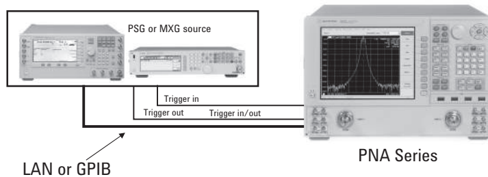
Figure 57. Configuring an external source.
