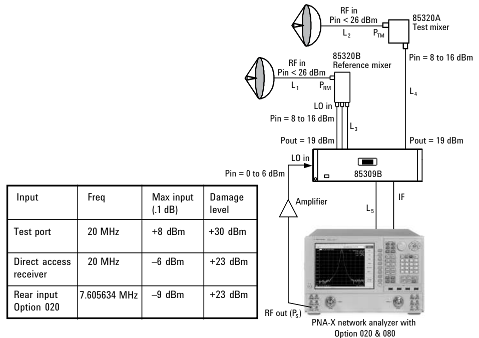
Figure 18. Receive site configuration with external mixing using the PNA-X N5242A network analyzer.
