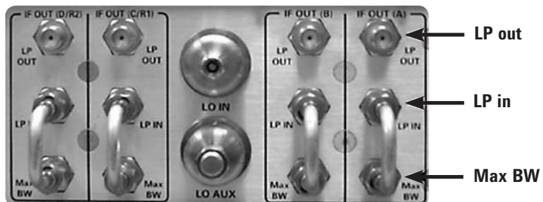
Figure 46. N5280A frequency converter rear panel detail.
