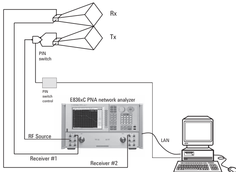
Figure 9. Typical RCS measurement configuration using a Legacy (E836xC) PNA network analyzer. PNA-L Option 216, PNA Option 201, or PNA-X can also be used.
