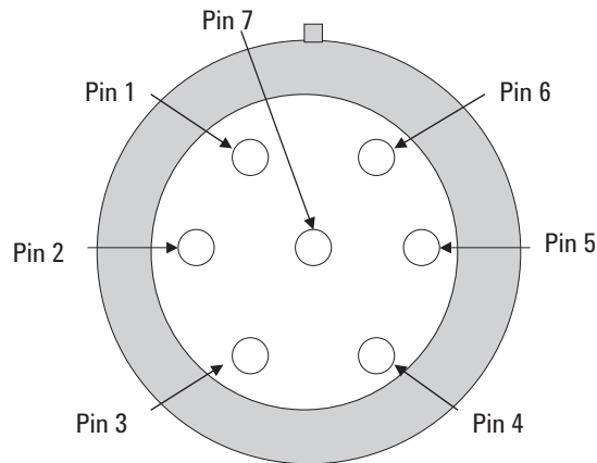
Figure 56. Bias connector pin locations (enlarged).
