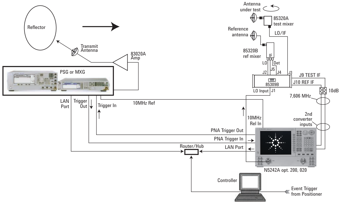
Figure 1. Simplified far-field antenna range example with MXG Source and N522xA PNA or N5264A PNA-X Measurement Receiver with LO source (Option 108).
