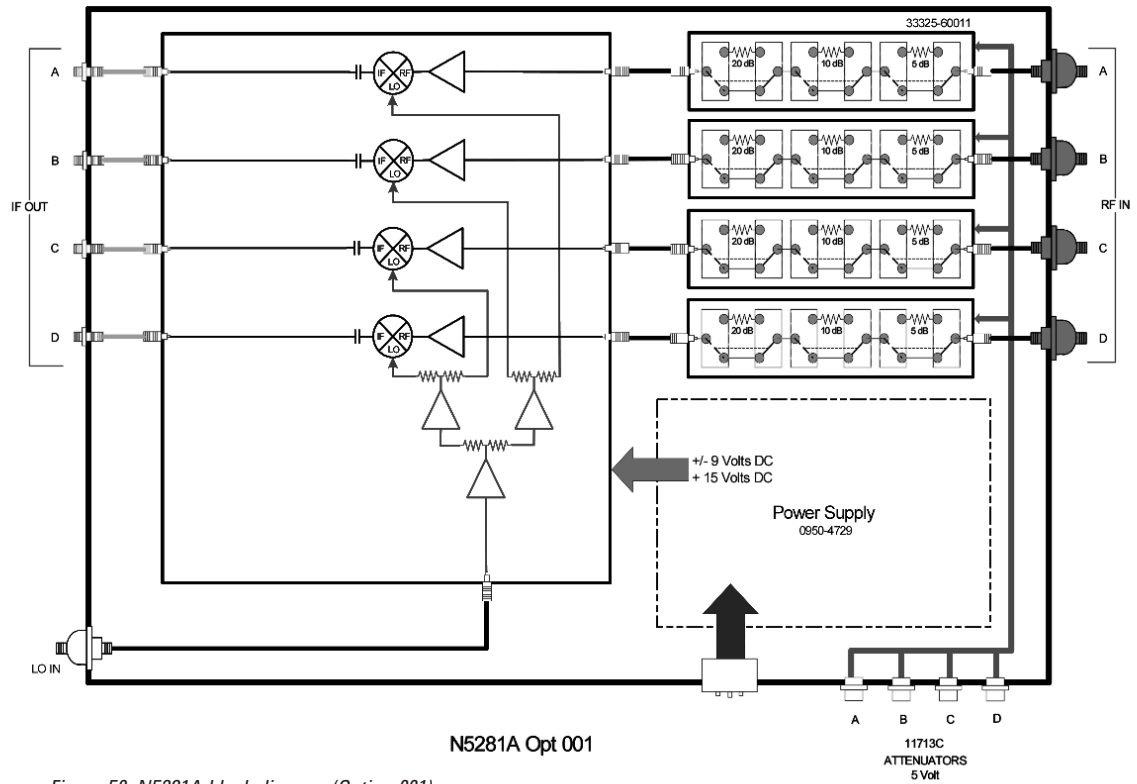
Figure 50. N5281A block diagram (Option 001)
