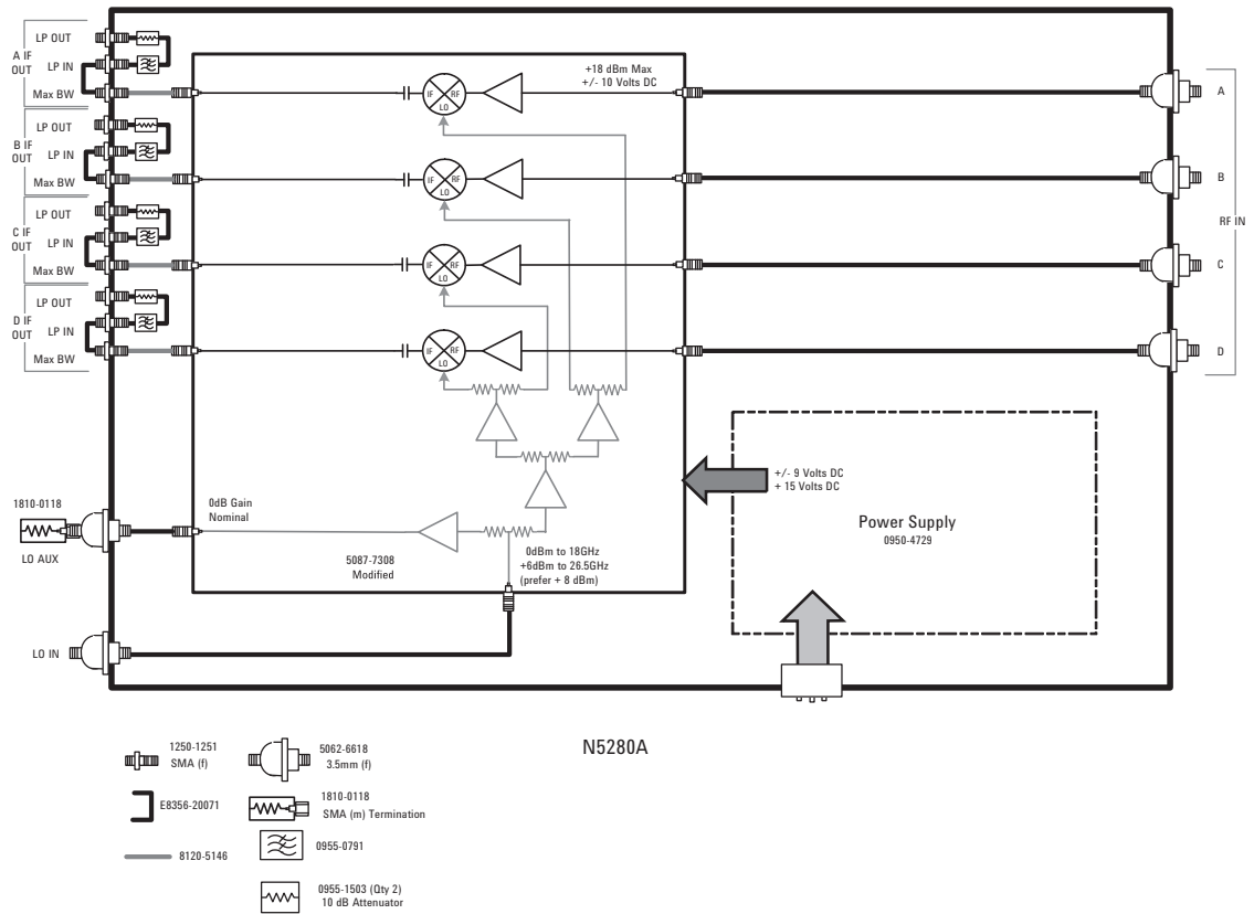
Figure 47. N5280A block diagram (Standard 700)
