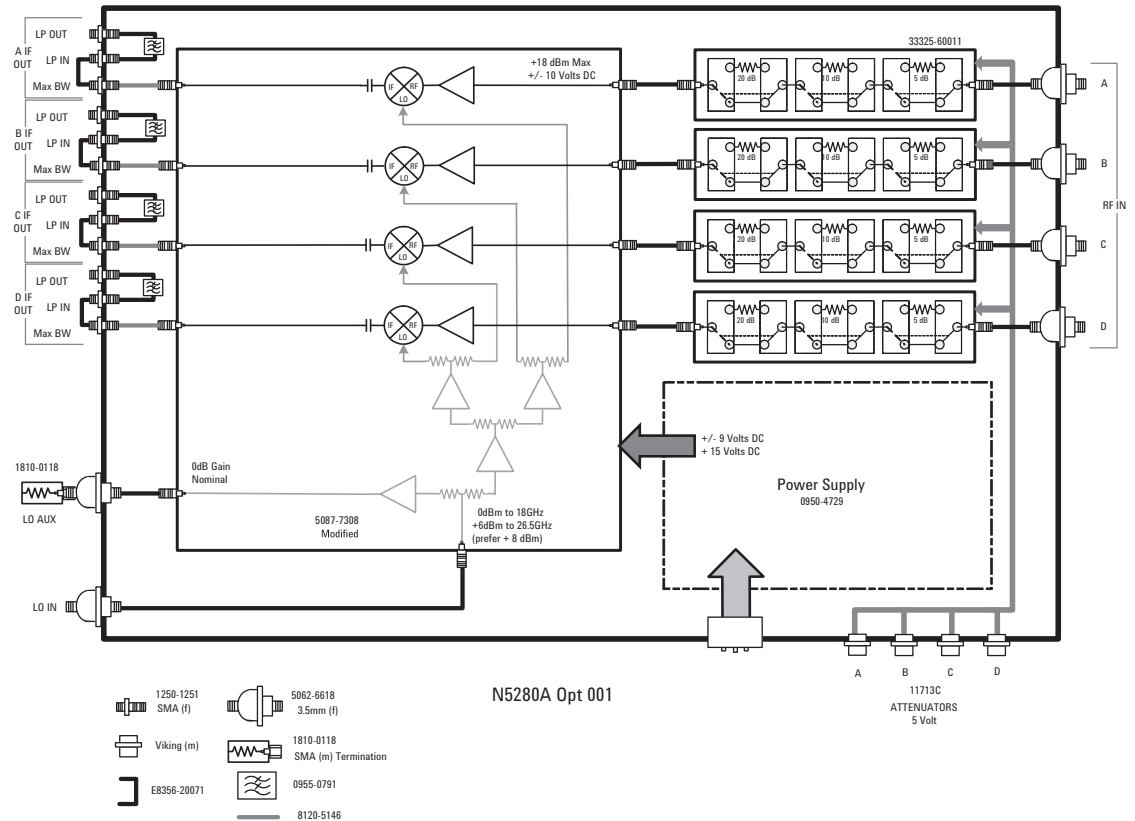
Figure 48. N5280A block diagram (Option 001)
