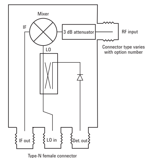
Figure 43. 85320B reference mixer.
