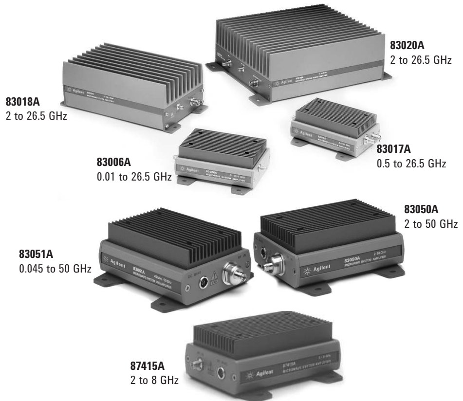
Figure 51. Amplifiers.
