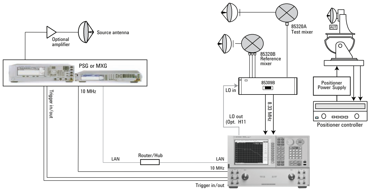
Figure 5. Typical antenna measurement configuration using PNA network analyzers with Option H11.
