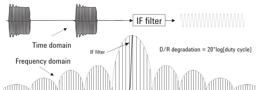
Figure 35. Time domain.
