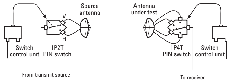
Figure 53. A typical multiple-channel, multiple-frequency system configuration.
