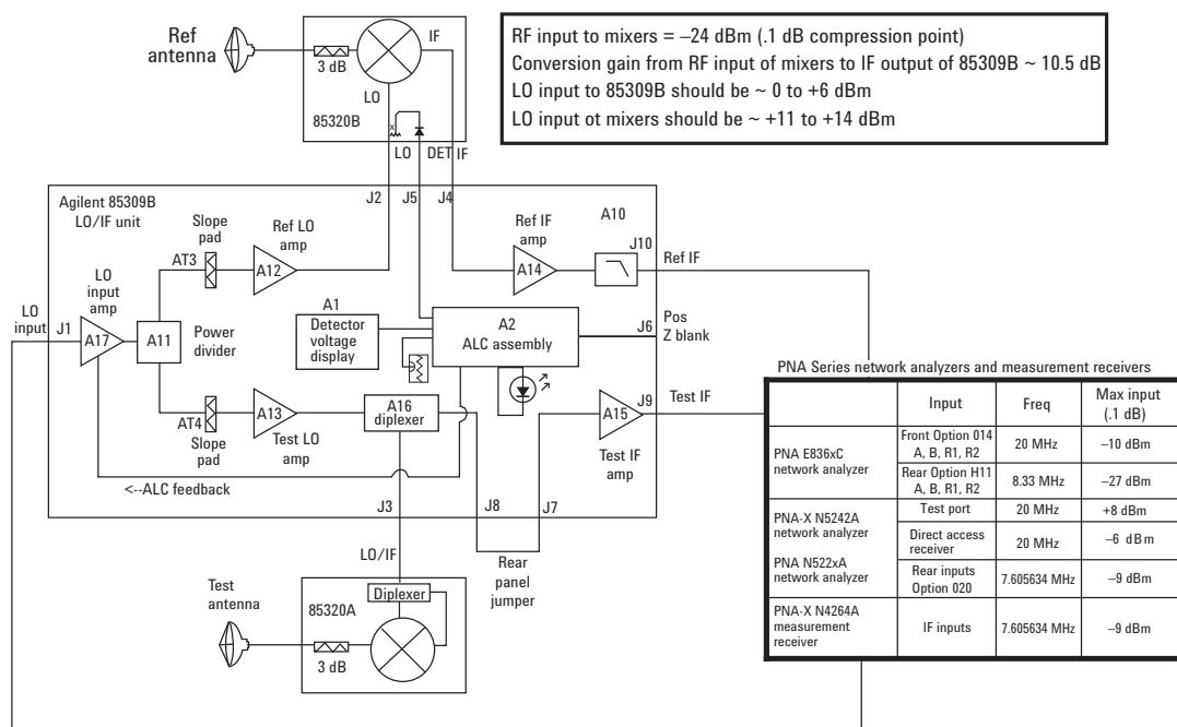
Figure 40. 85309B LO/IF distribution unit block diagram.
