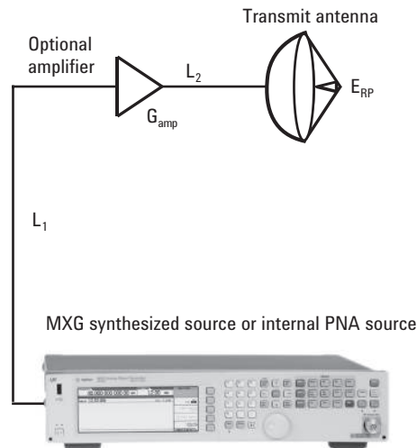
Figure 14. Transmit site configuration.
