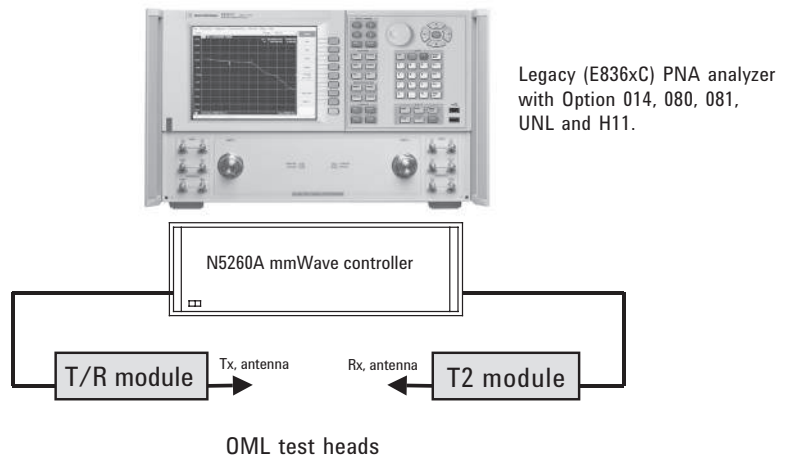
Figure 11. Typical millimeter-wave configuration using an Agilent PNA, a mm-wave controller and Oleson Microwave Laboratory mm-wave modules.
