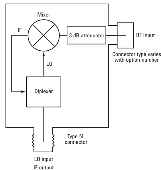
Figure 42. 85320A test mixer.
