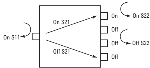
Figure 55. Switch port match definitions for switch on/off states.
