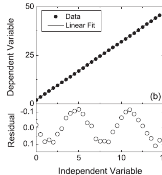
Fig. 5.9 The least-squares best-fit straight line to a sinusoidal variation. Error bars smaller than symbol size. Health warning It is possible to use the method of least squares to find the 'best-fit' straight line for any data set. This does not mean that a linear fit is an appropriate theoretical model.
