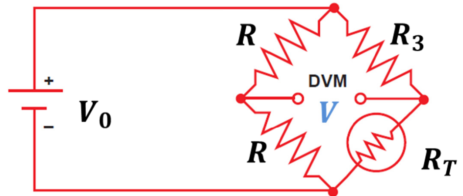
WHEATSTONE BRIDGE
